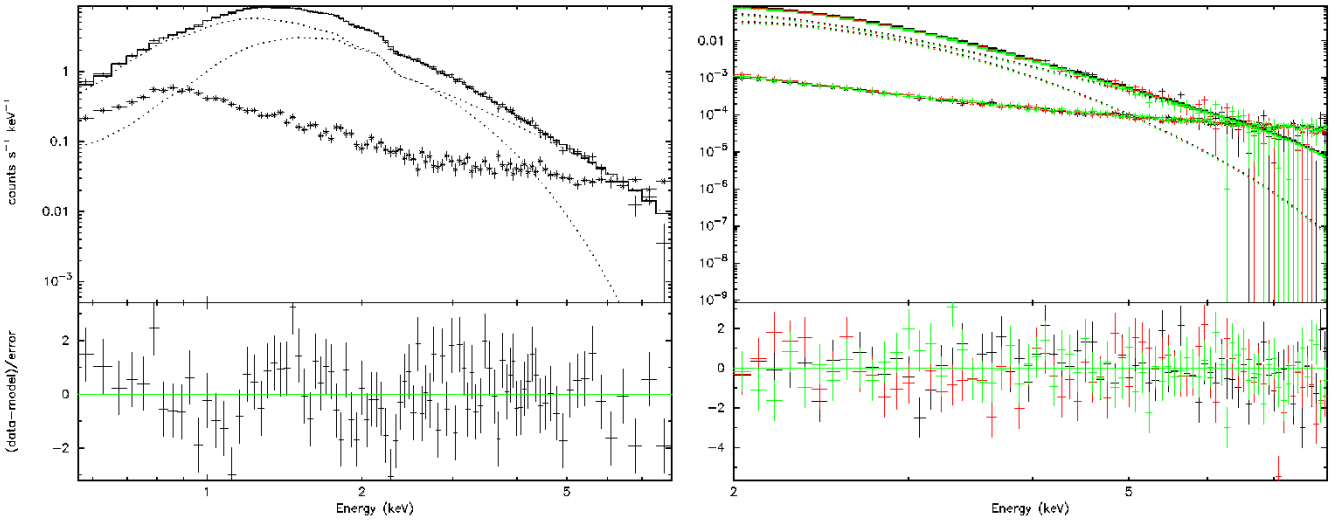
Figure 4. Left: spectral fit of the EPIC-pn XMM-Newton data with the \text{phabs} \times (\text{bbodyrad} + \text{powerlaw}) \times \text{gabs} model in the 0.5–8 keV range. Right: same for the IXPE DU1 (black), DU2 (red) and DU3 (green) data in the 2–8 keV range. The single spectral components are marked by dotted lines (see also Table 2) and the background counts by crosses with error bars.
