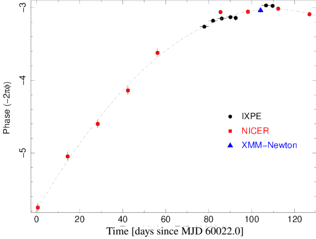
Figure 1. 1E 2259+586 phase evolution (in radian units) as a function of time fitted with a linear plus a quadratic component for the whole data sample used in the analysis, that includes IXPE (black filled circles), NICER (red filled squares) and XMM-Newton (blue filled triangles). The dash-dotted line marks the best fit.
