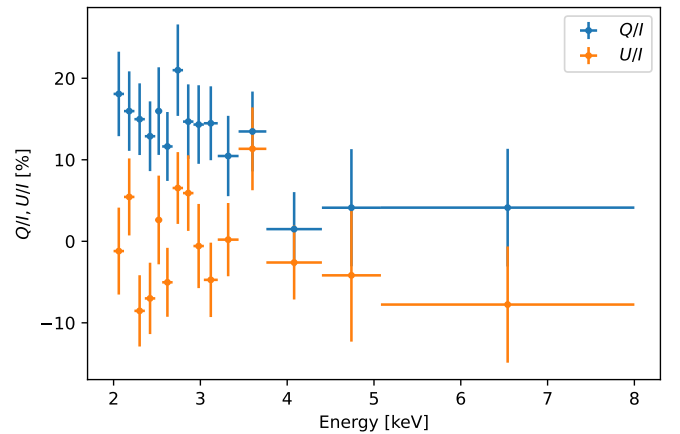
Figure 11. Normalized Stokes parameters Q/I and U/I plotted as functions of energy, referred to the frame of the best-fitting RVM with mode switching (dashed curve in Figure 7).
